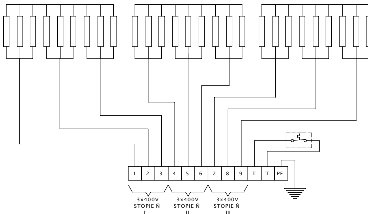
Fig. No 29 Connection of grilles in heater 324-3
