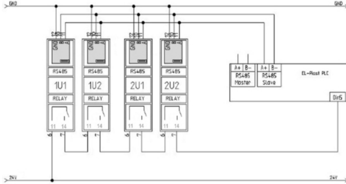
Rys Nr 19 Example for double supply, double exhaust
