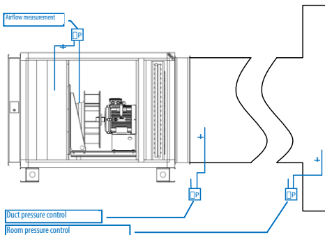
Fig. No 8 Other possible pressure measurements with transmitters depending on their installation
