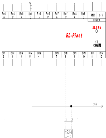
Fig. No 2 Additional pressure switch on fine filter or electrostatic filter alarm contact
