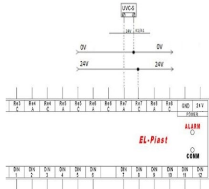
Fig. No 5 Connection of UVC-S lamp control
