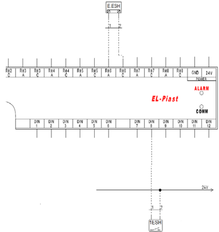
Fig. No 4 Monitoring the operation of the electrostatic filter
