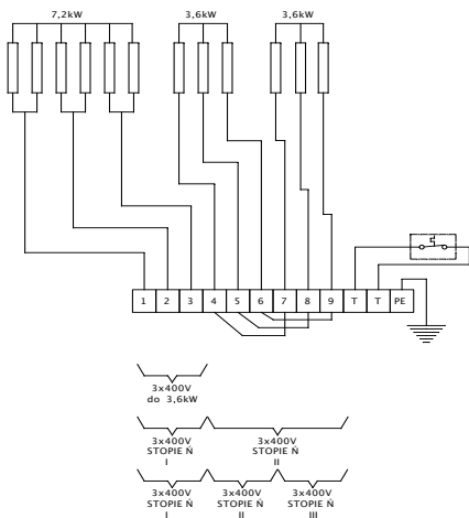
Fig. No 27 Connection of grilles in heater 144-2
