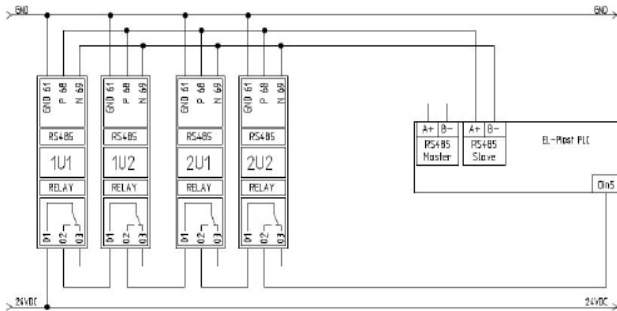
Fig. No 15 Example for double supply, double exhaust
