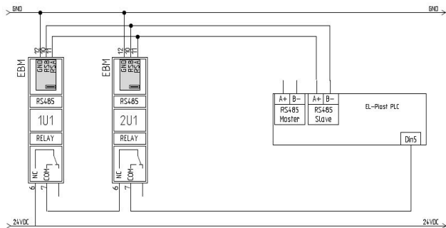
Fig. No18 Example for single supply, single exhaust.
