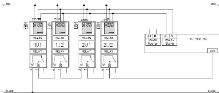
Fig. No 17 Example for double supply, double exhaust
