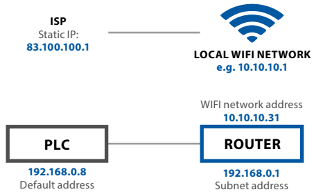
Fig. 17 Connecting the controller with the local WIFI network with external sharing
