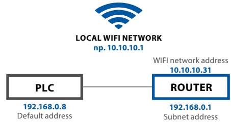
Fig. 15 Connecting the controller to a local network via WIFI
